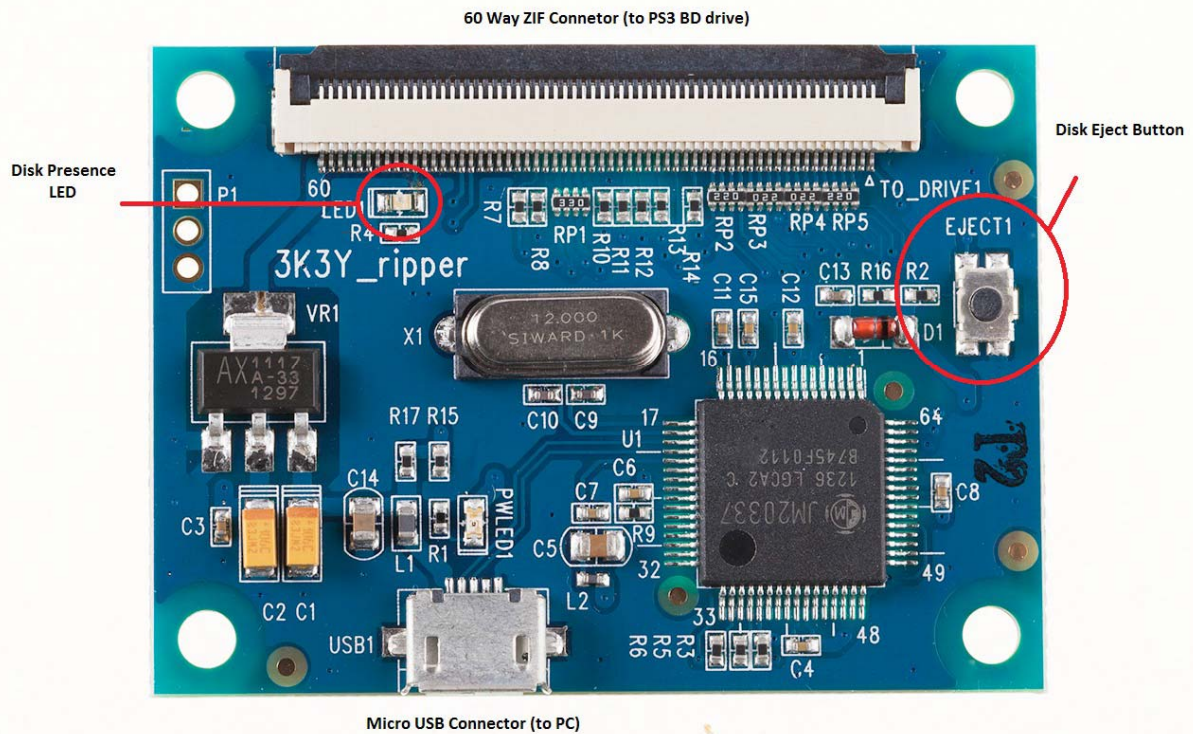
Figure 1 : PCB 3K3Y Ripper PCB
